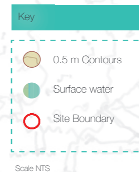
Fig 6: Landform
